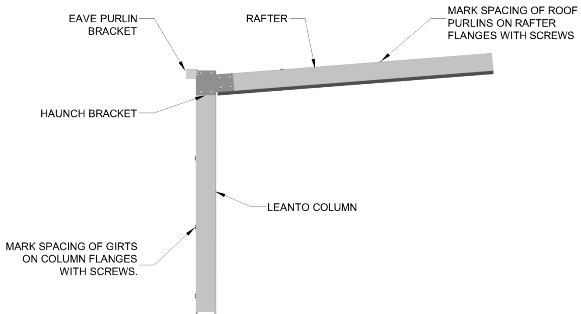
HAUNCH BRACKET FITTED TO RAFTER
