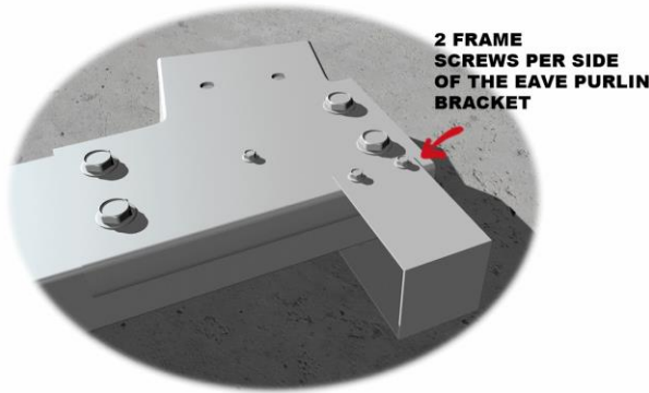
SINGLE COLUMN EAVE PURLIN BRACKET CONNECTION
