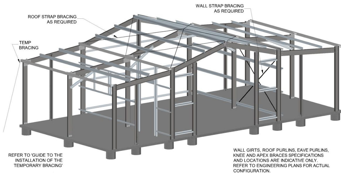
FIXING OF LEANTO ROOF PURLIN - Z SECTION
