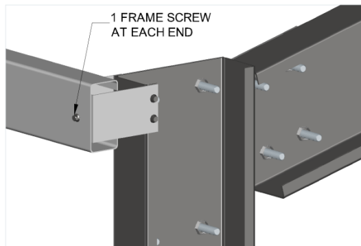
EAVE PURLIN CONNECTION AT END WALL COLUMN
