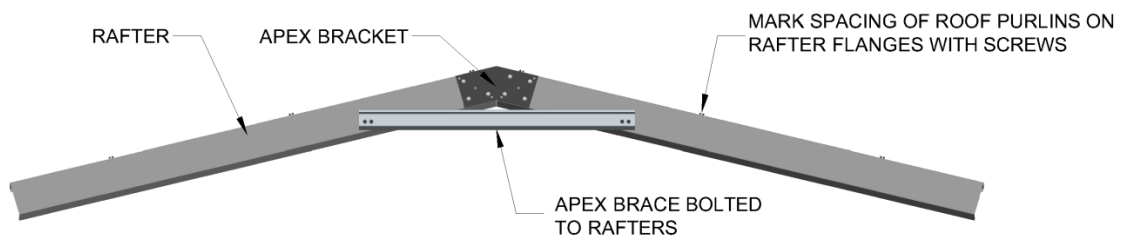
RAFTERS FITTED WITH APEX BRACE
