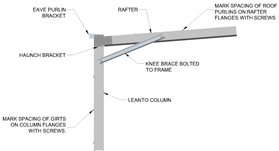
KNEE BRACE FITTED TO COLUMN AND RAFTER (COMPLETE LEANTO PORTAL FRAME ASSEMBLY)
