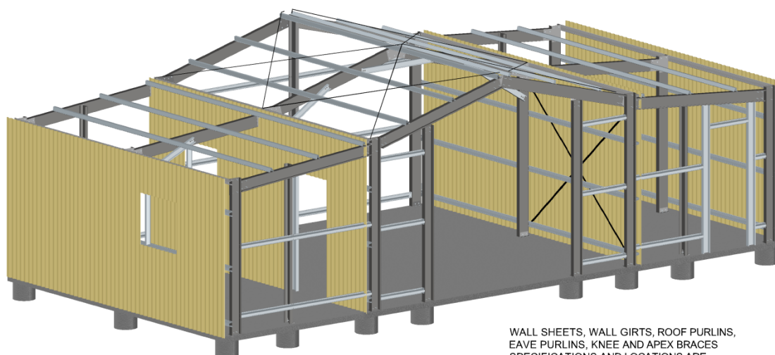
FIXING OF MAIN SIDE WALL SHEETS
