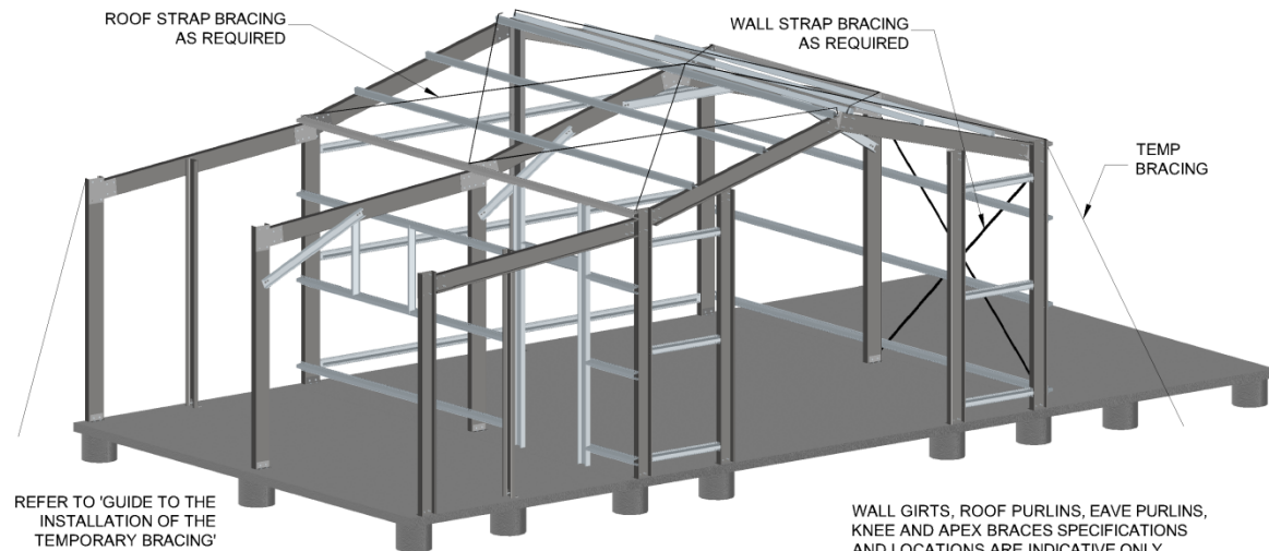
STANDING ALL LEFT LEANTO PORTAL FRAME ASSEMBLY
