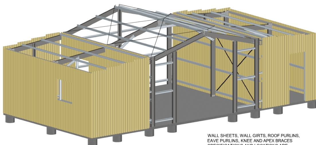
FIXING OF LEAN-TO END WALL SHEETS
