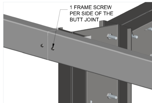
EAVE PURLIN CONNECTION AT INTERMEDIATE COLUMN
