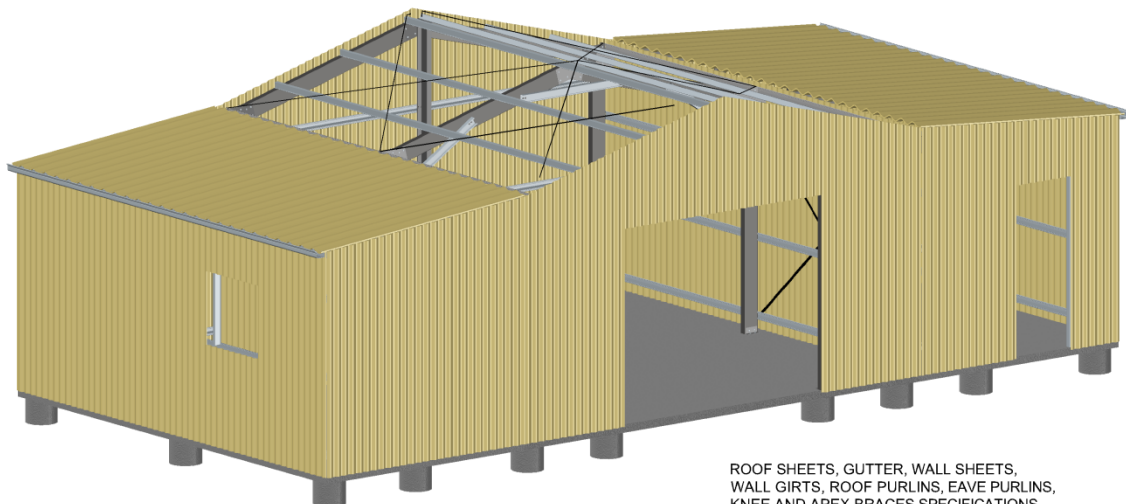
FIXING OF LEAN-TO ROOF SHEETS
