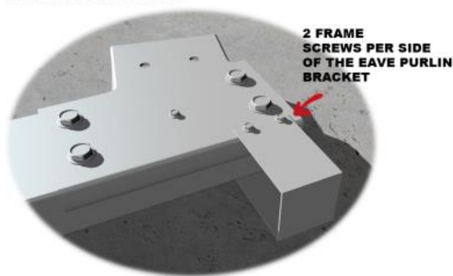
SINGLE COLUMN EAVE PURLIN BRACKET CONNECTION
