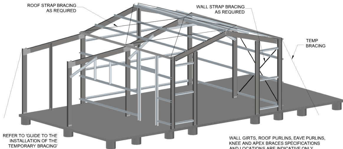
STANDING THE SECOND LEFT LEANTO PORTAL FRAME ASSEMBLY
