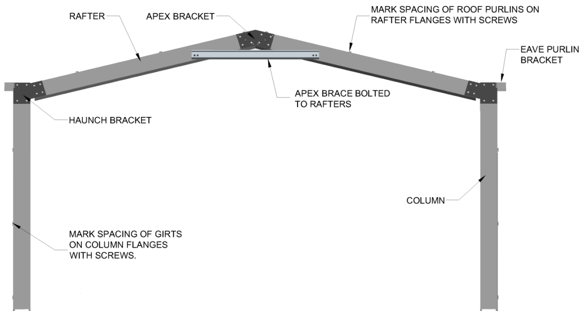
HAUNCH BRACKET FITTED TO RAFTERS
