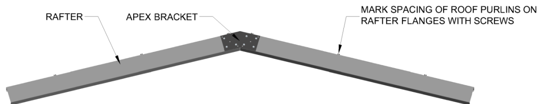
RAFTERS FITTED WITH APEX BRACKET
