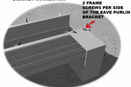
DOUBLE COLUMN EAVE PURLIN BRACKET CONNECTION
