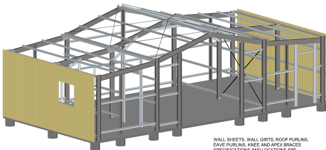
FIXING OF LEAN-TO SIDE WALL SHEETS
