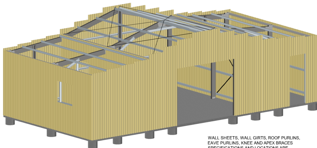
FIXING OF MAIN END WALL SHEETS
